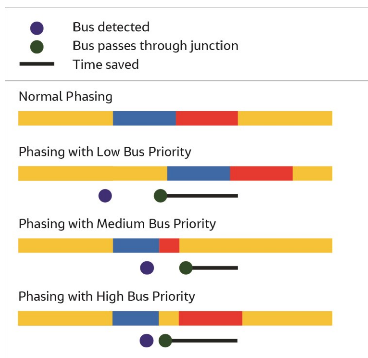
Diagram 7.2 Principles for high, medium and low bus priority
