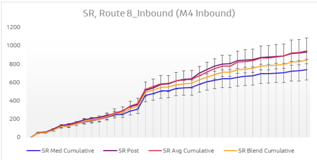
Diagram 6.16 Journey Time Validation Plot - Route 8 Inbound SR
