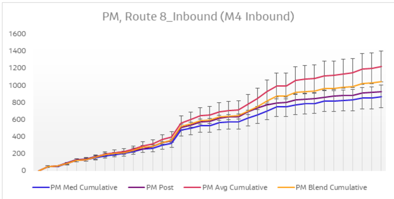
Diagram 6.18 Journey Time Validation Plot - Route 8 Inbound PM
