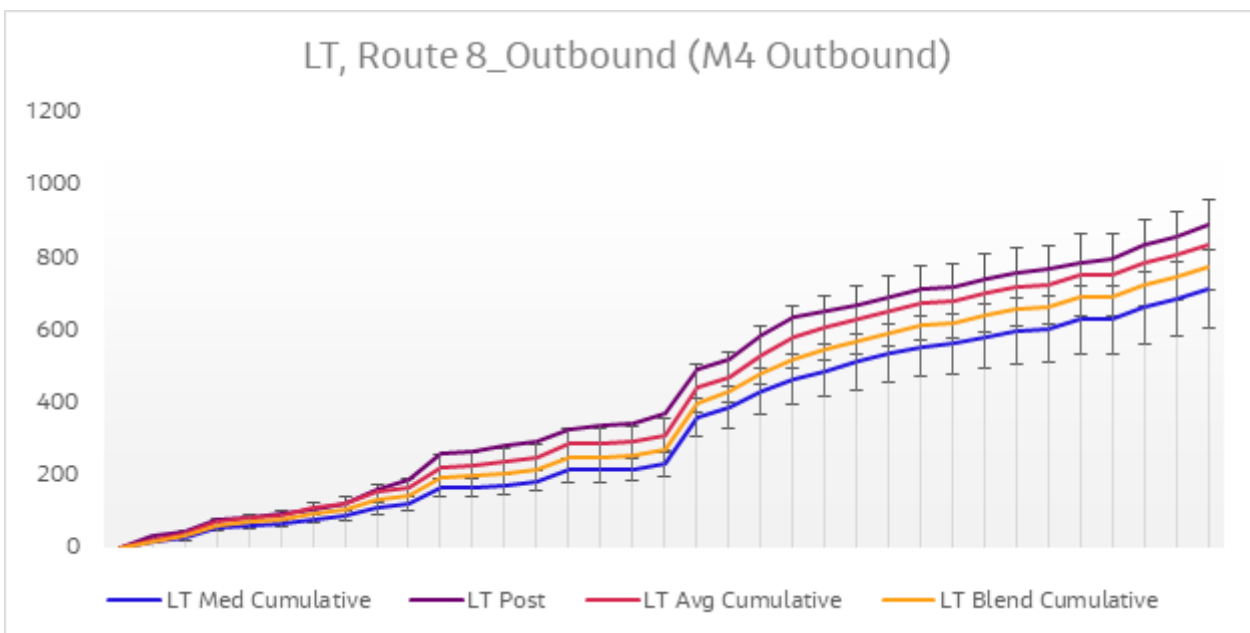
Diagram 6.15 Journey Time Validation Plot - Route 8 Outbound LT
