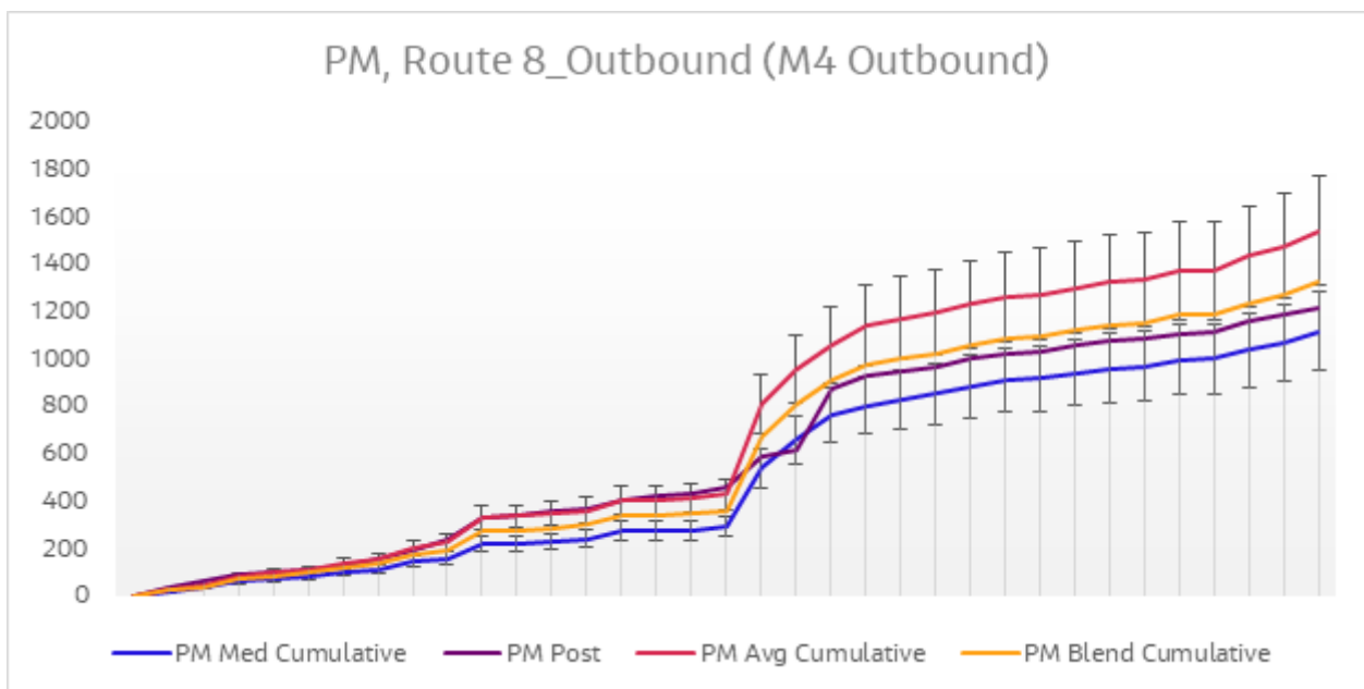
Diagram 6.19 Journey Time Validation Plot - Route 8 Outbound PM
