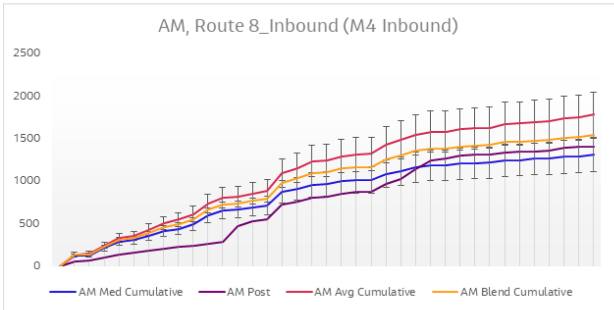
Diagram 6.12 Journey Time Validation Plot – Route 8 Inbound AM
