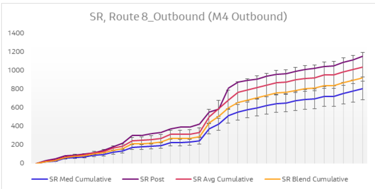
Diagram 6.17 Journey Time Validation Plot - Route 8 Outbound SR
